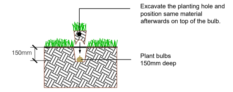
Bulb planting Scale 1:20 (A1)
