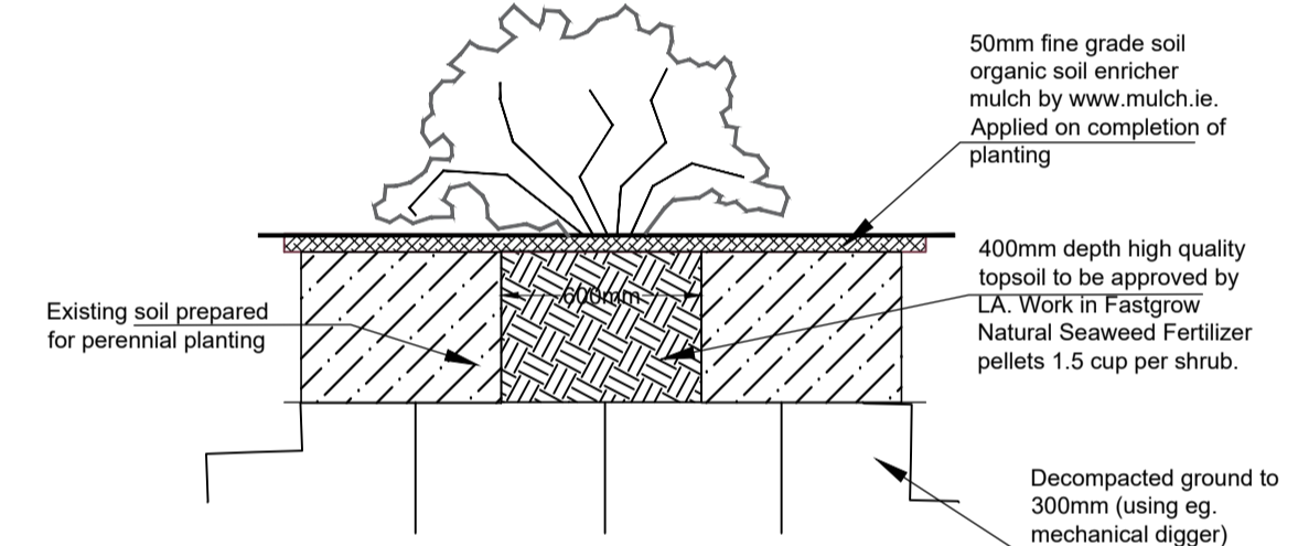
Shrub Planting Scale 1:20 (A1)
