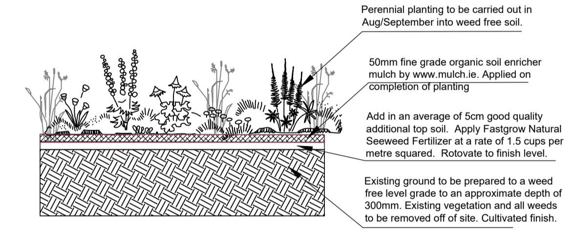
Soil preparation for planting beds Scale 1:20 (A1)
